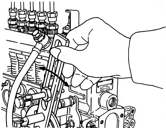
Fig. 67 Checking control rack movement
